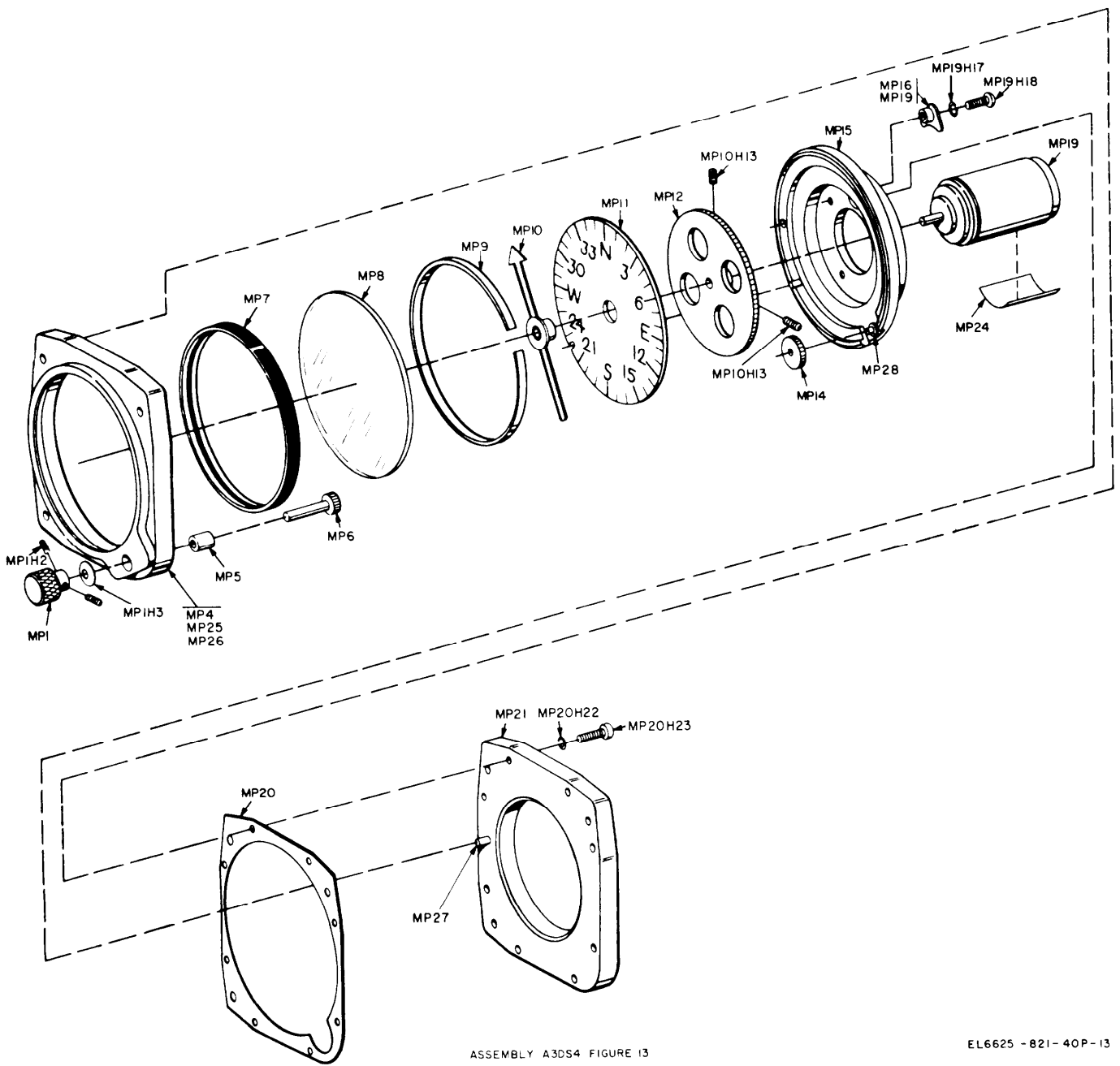
ASSEMBLY A3DS4 FIGURE 13
