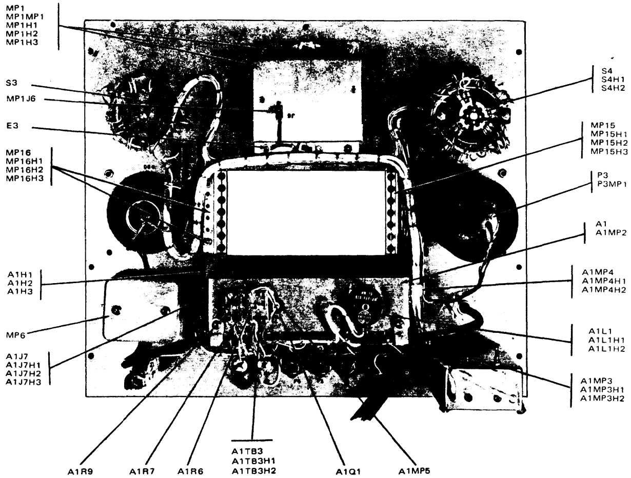
ASSEMBLY A3 FIGURE 7
