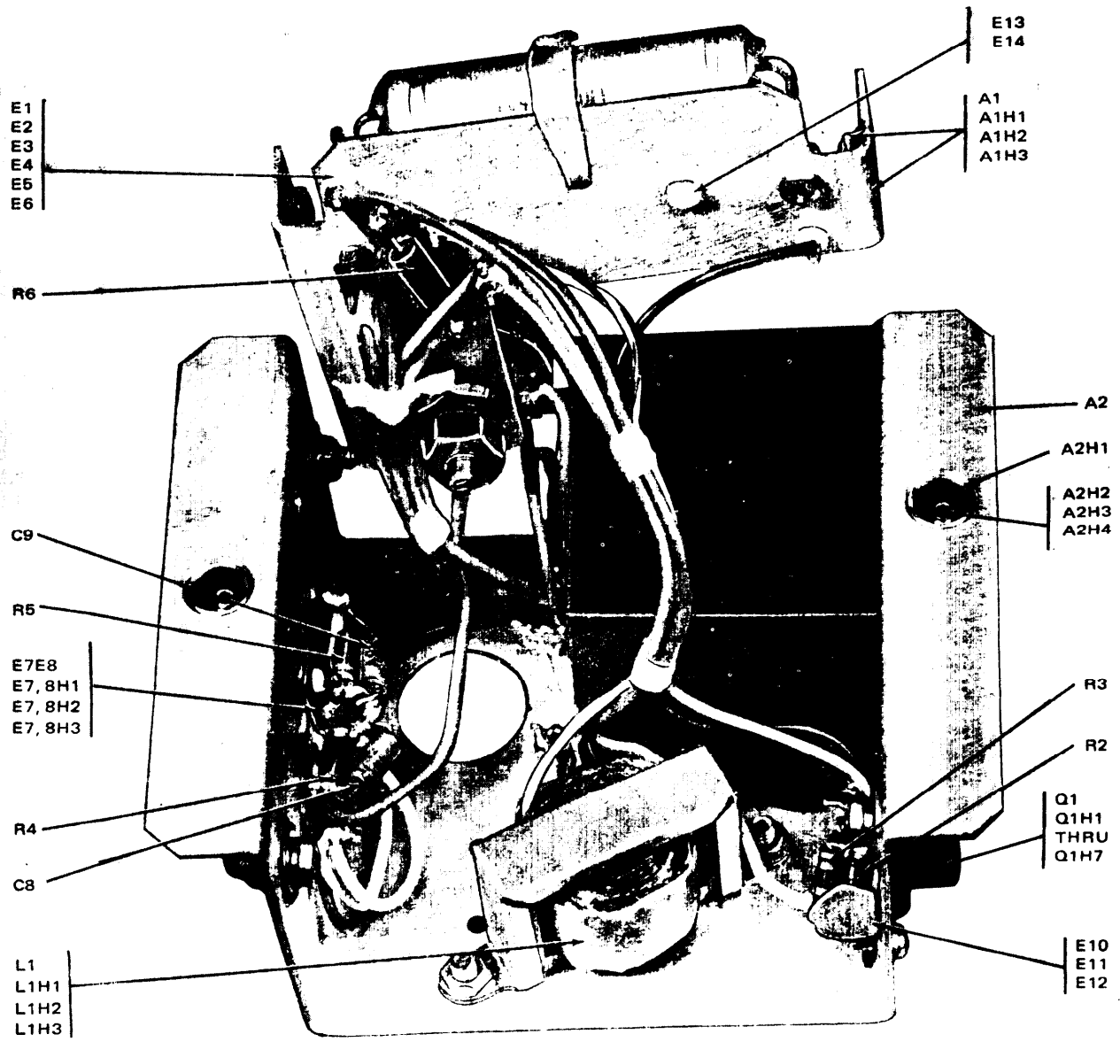
ASSEMBLY A3A2 FIGURE 12
