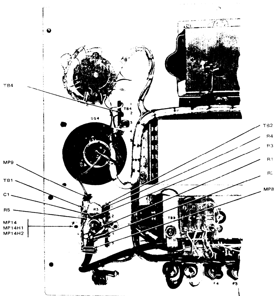
ASSEMBLY A3 FIGURE 9
