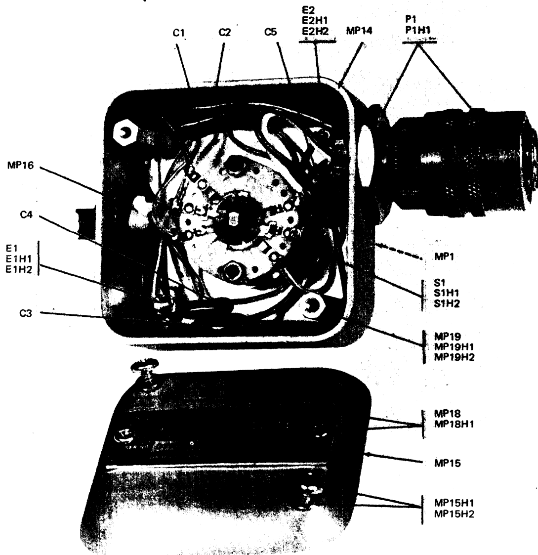
ASSEMBLY A2 FIGURE 5
