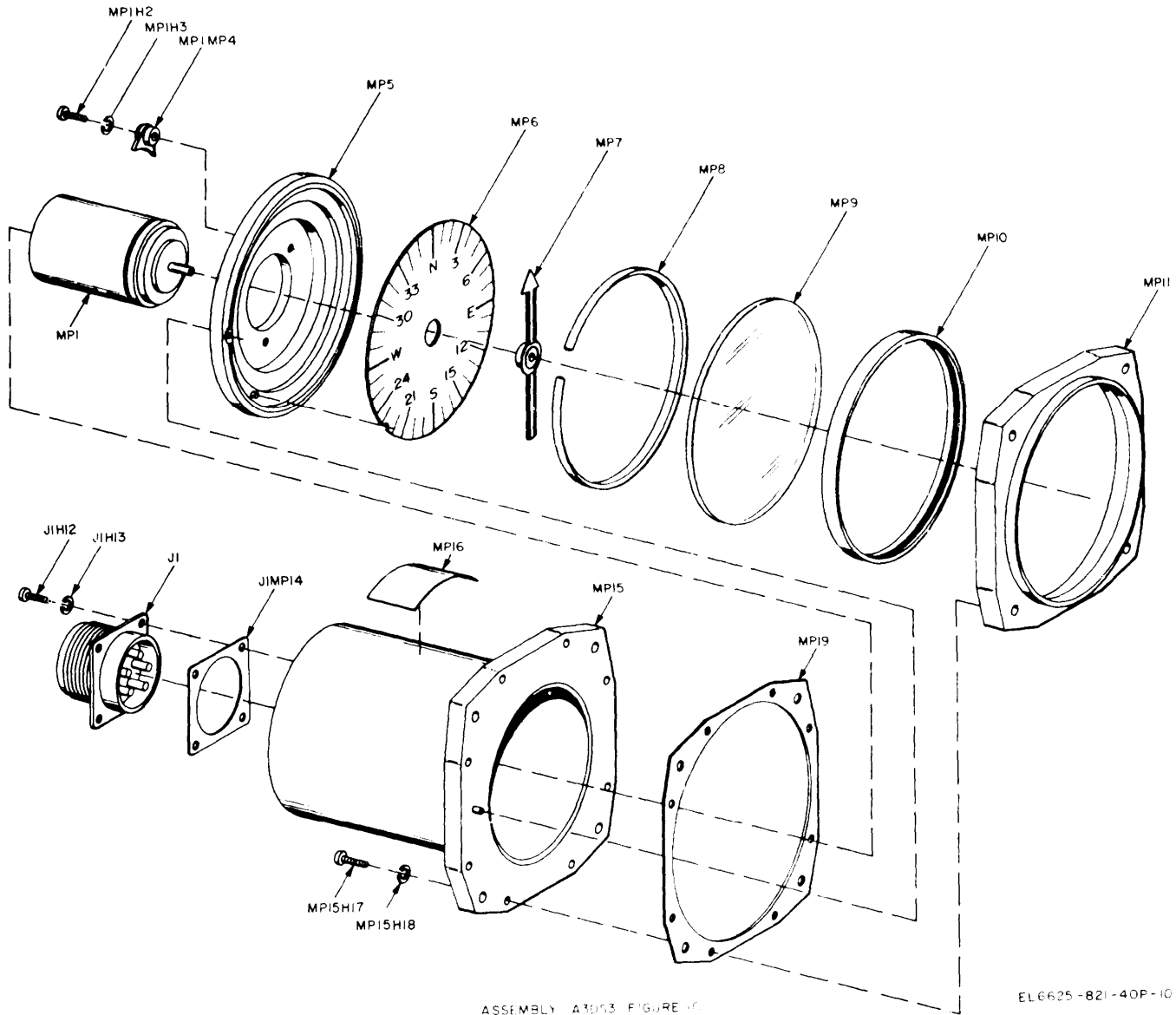
ASSEMBLY A3013 FIGURE 10
