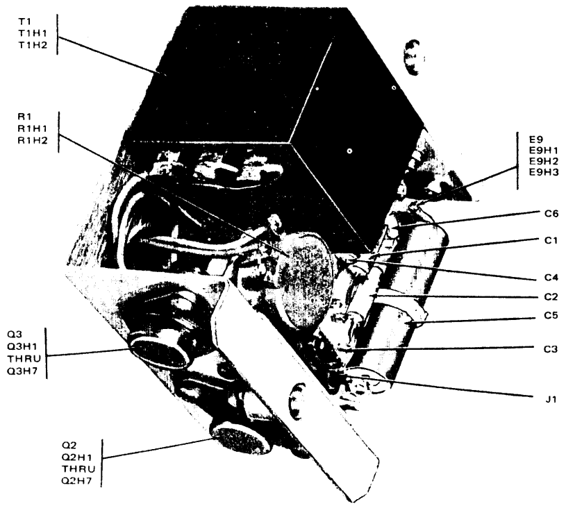
ASSEMBLY A3A2 FIGURE 11
